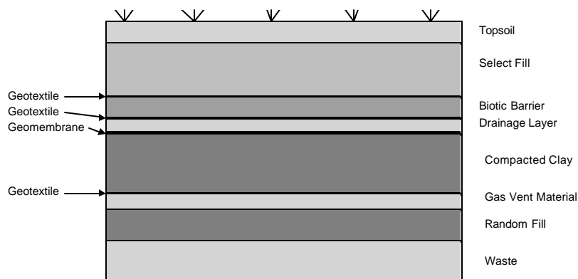
Figure B-1. Landfill cover with all optional layers.
